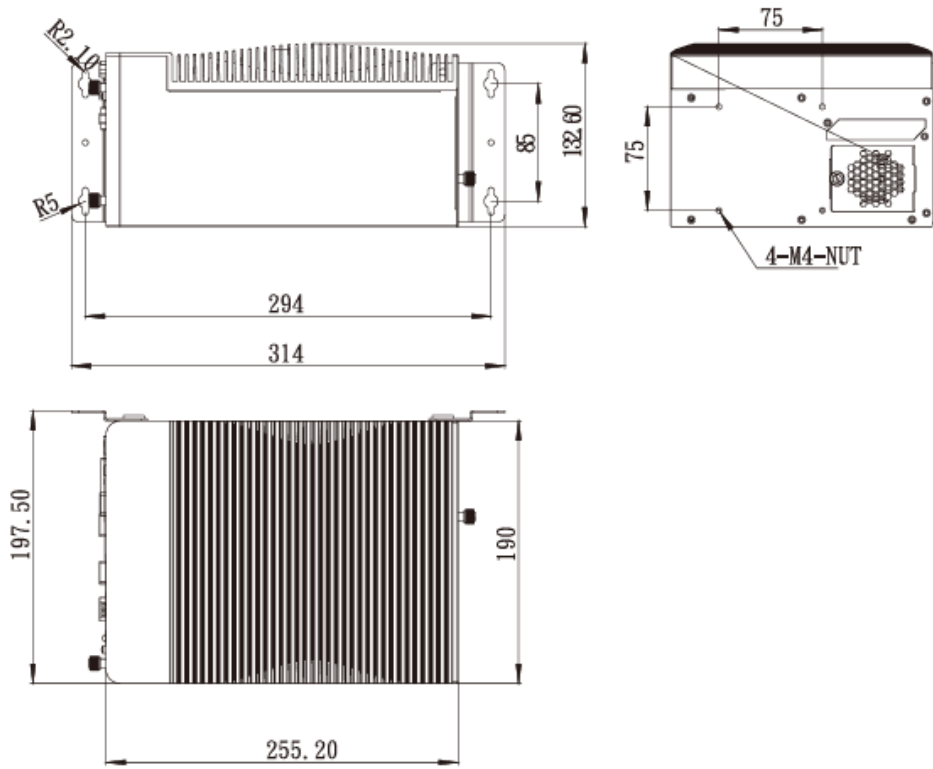
Figure 1-6: TANK-870e-H110 Physical Dimensions (millimeters)
