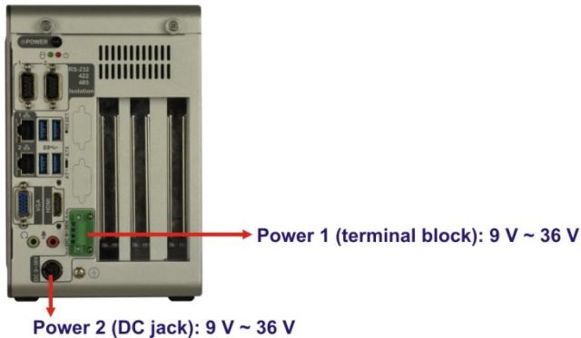
Figure 3-16: Power Connectors
