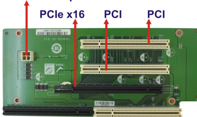
Figure 1-4: HPE-3S6
