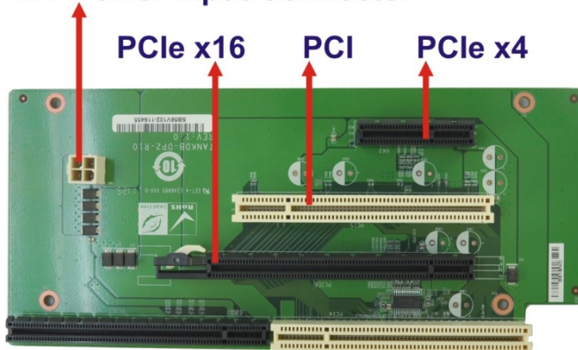
Figure 1-5: HPE-3S7
