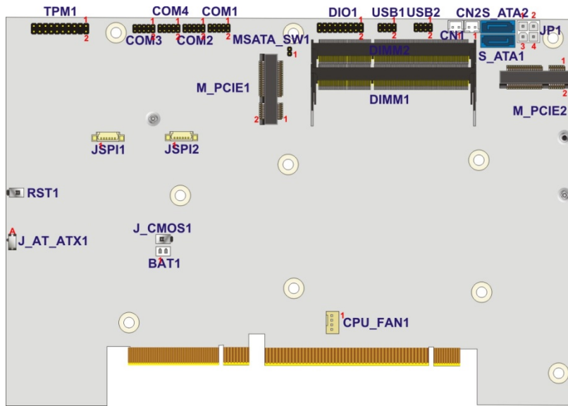
Figure 4-1: System Motherboard (Front)
