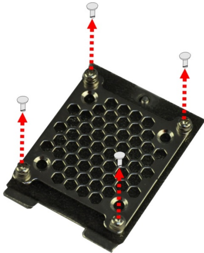
Figure 3-6: Remove the Fan Bracket from the Cover
