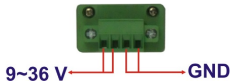
Figure 3-13: 4-pin Terminal Block
