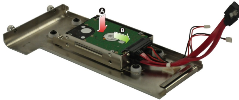
Figure 3-3: HDD Installation
