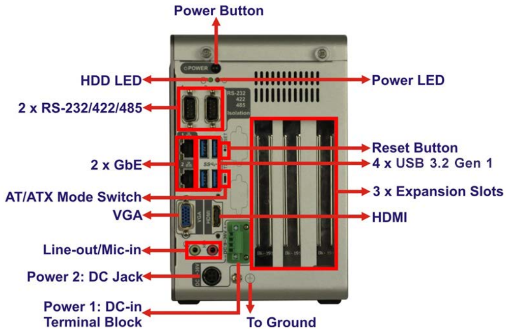
Figure 1-2: TANK-870e-H110 Front Panel
