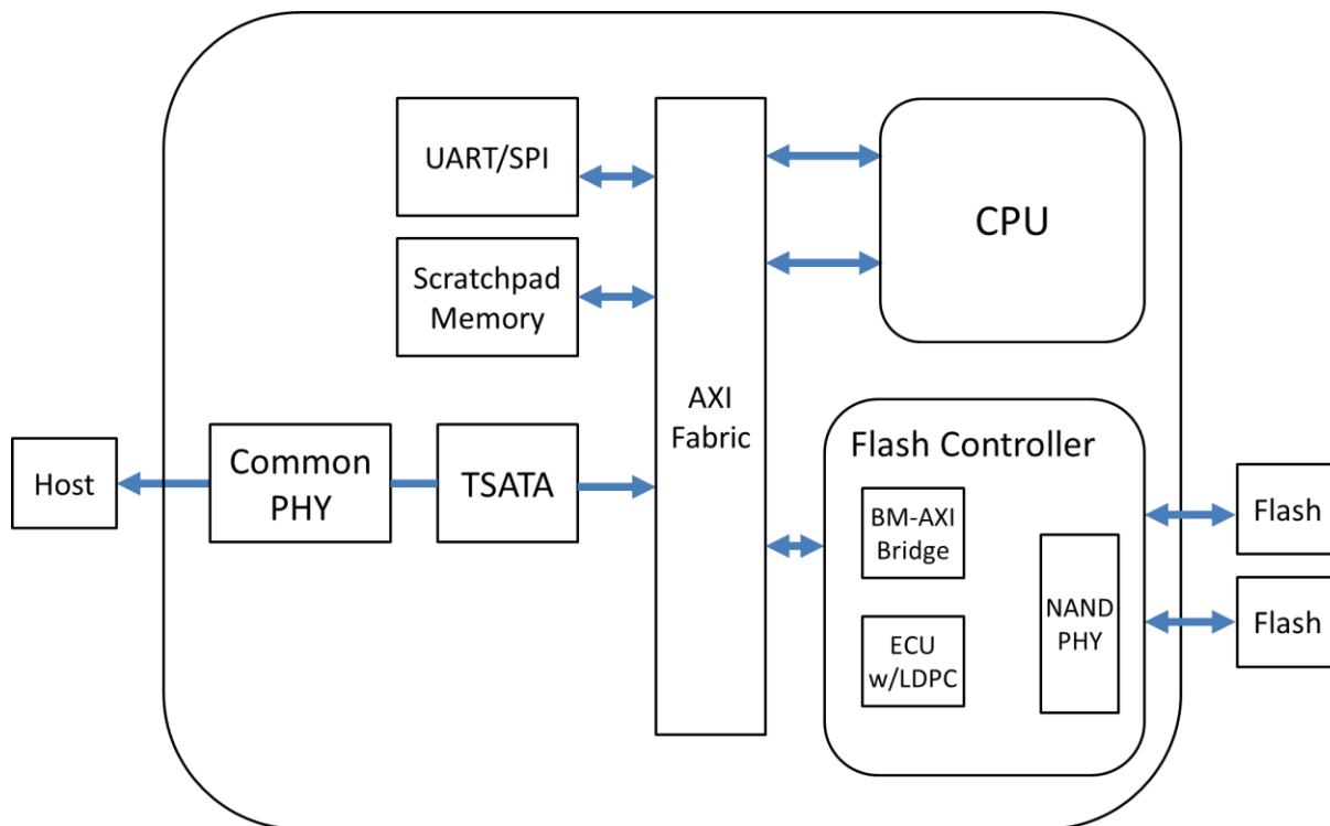
Figure 3: Innodisk SATADOM-SV 3IE4 Block Diagram
