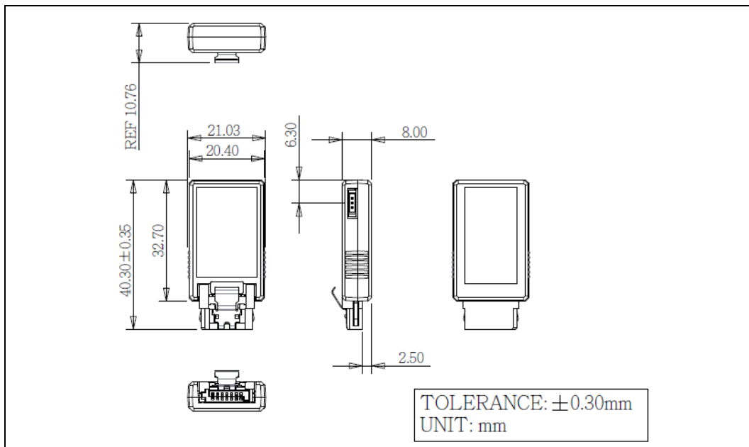
Figure 2: Innodisk SATADOM-SV 3IE4 Mechanical Diagram
