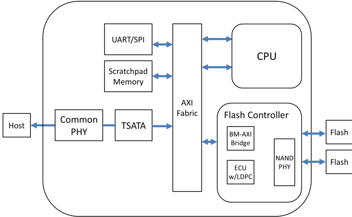
Figure 3: Innodisk SATADOM-MV 3IE4 Block Diagram
