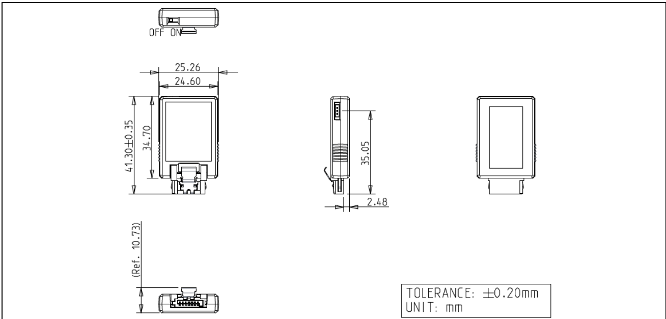
Figure 2: Innodisk SATADOM-MV 3IE4 mechanical diagram
