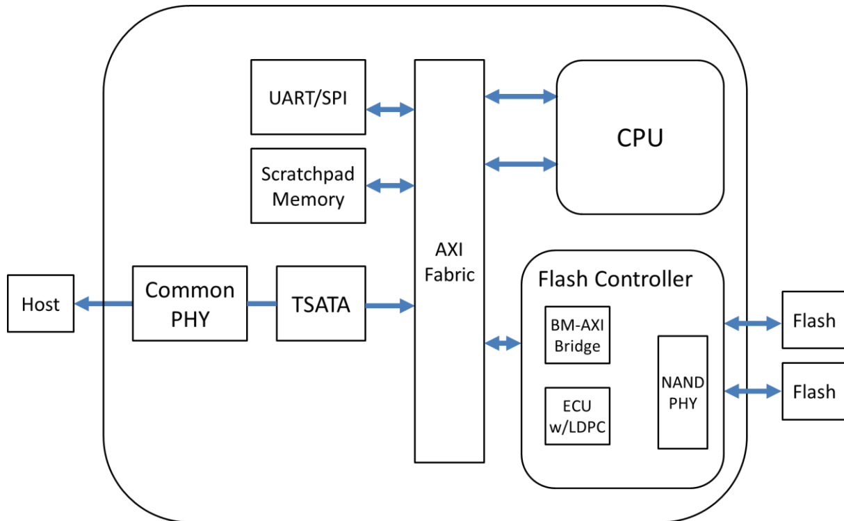
Figure 3: Innodisk SATADOM-MV 3ME4 Block Diagram
