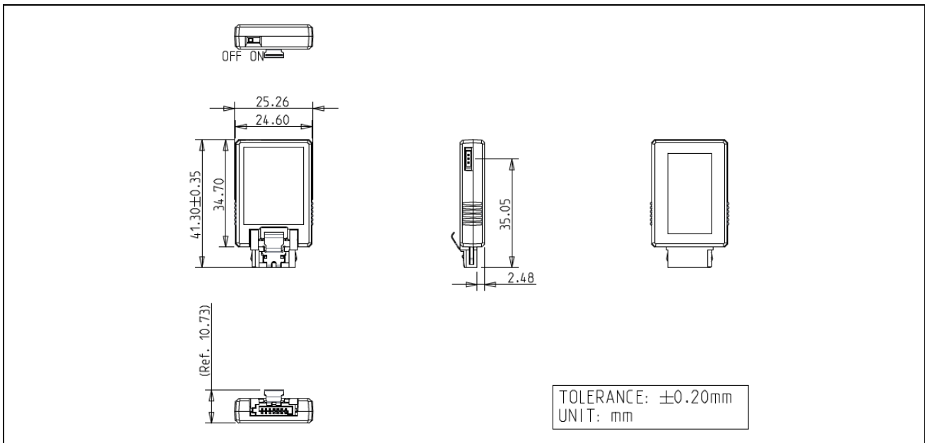
Figure 2: Innodisk SATADOM-MV 3ME4 mechanical diagram
