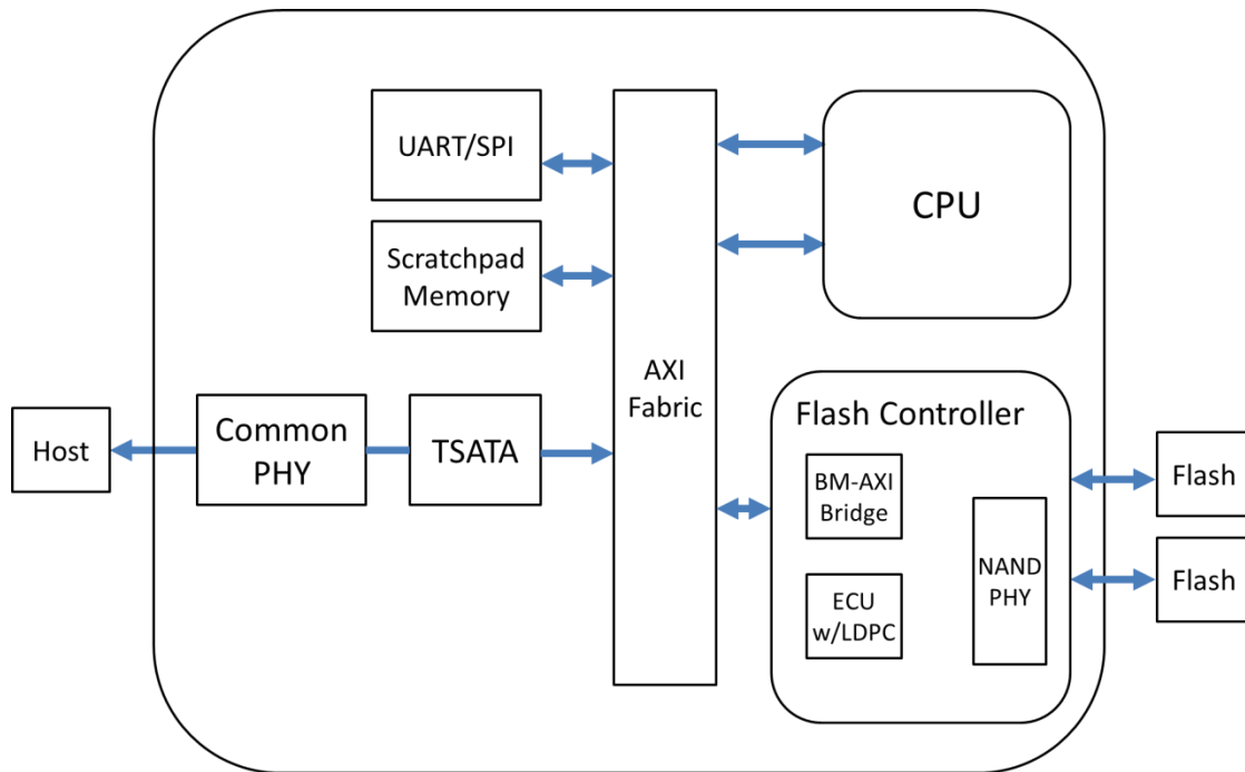
Figure 3: Innodisk SATADOM-SL 3ME4 Block Diagram
