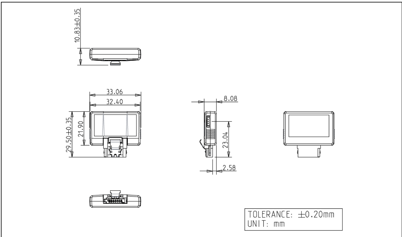
Figure 2: Innodisk SATADOM-SL 3ME4 mechanical diagram
