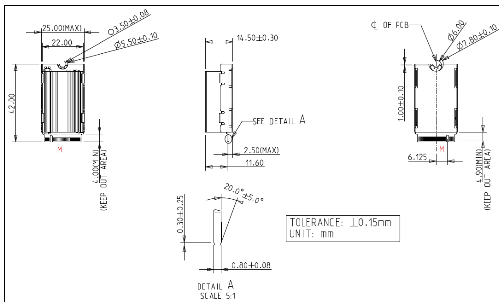
Figure 3: Innodisk M.2 (P42) 4TE2 mechanical drawing with heatsink diagram
