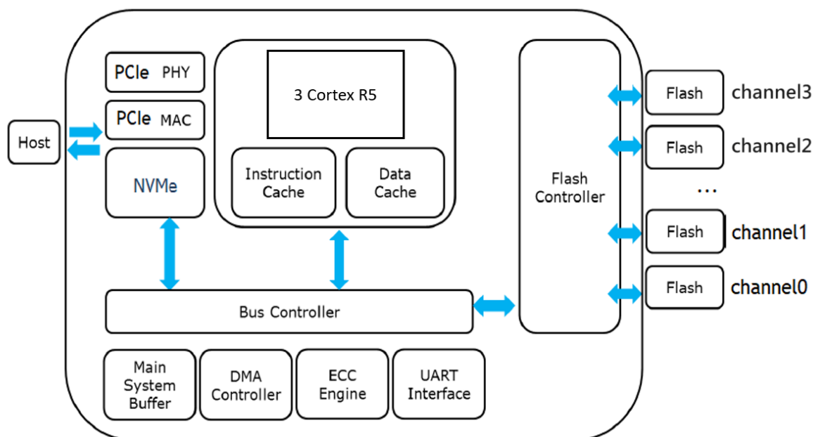
Figure 4: Innodisk M.2 (P42) 4TE2 Block Diagram
