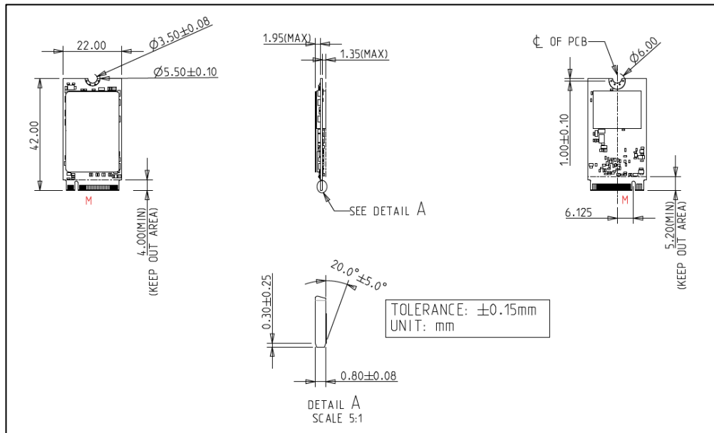
Figure 2: Innodisk M.2 (P42) 4TE2 mechanical drawing with CU Foil diagram
