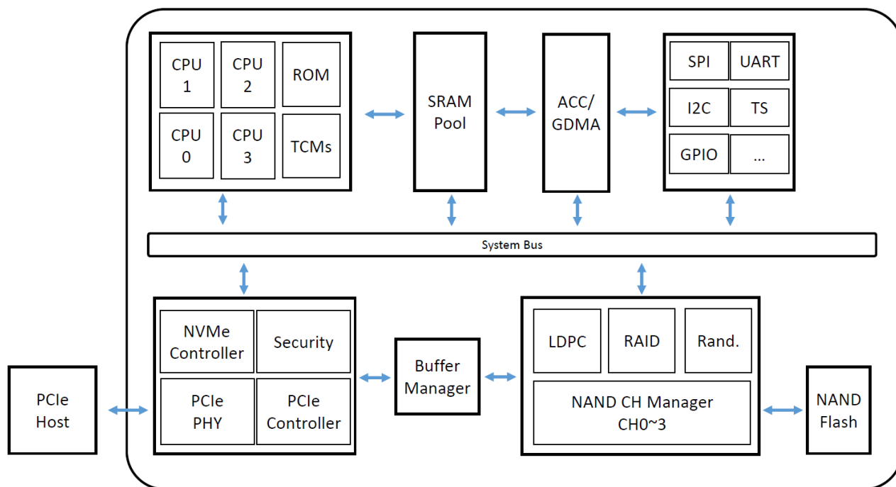
Figure 3: Innodisk M.2 (P80) 4IE3 Block Diagram
