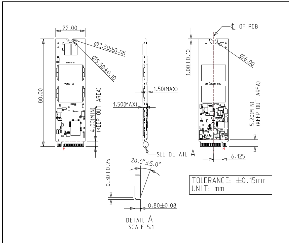
Figure 2: Innodisk M.2 (P80) 4IE3 mechanical drawing
