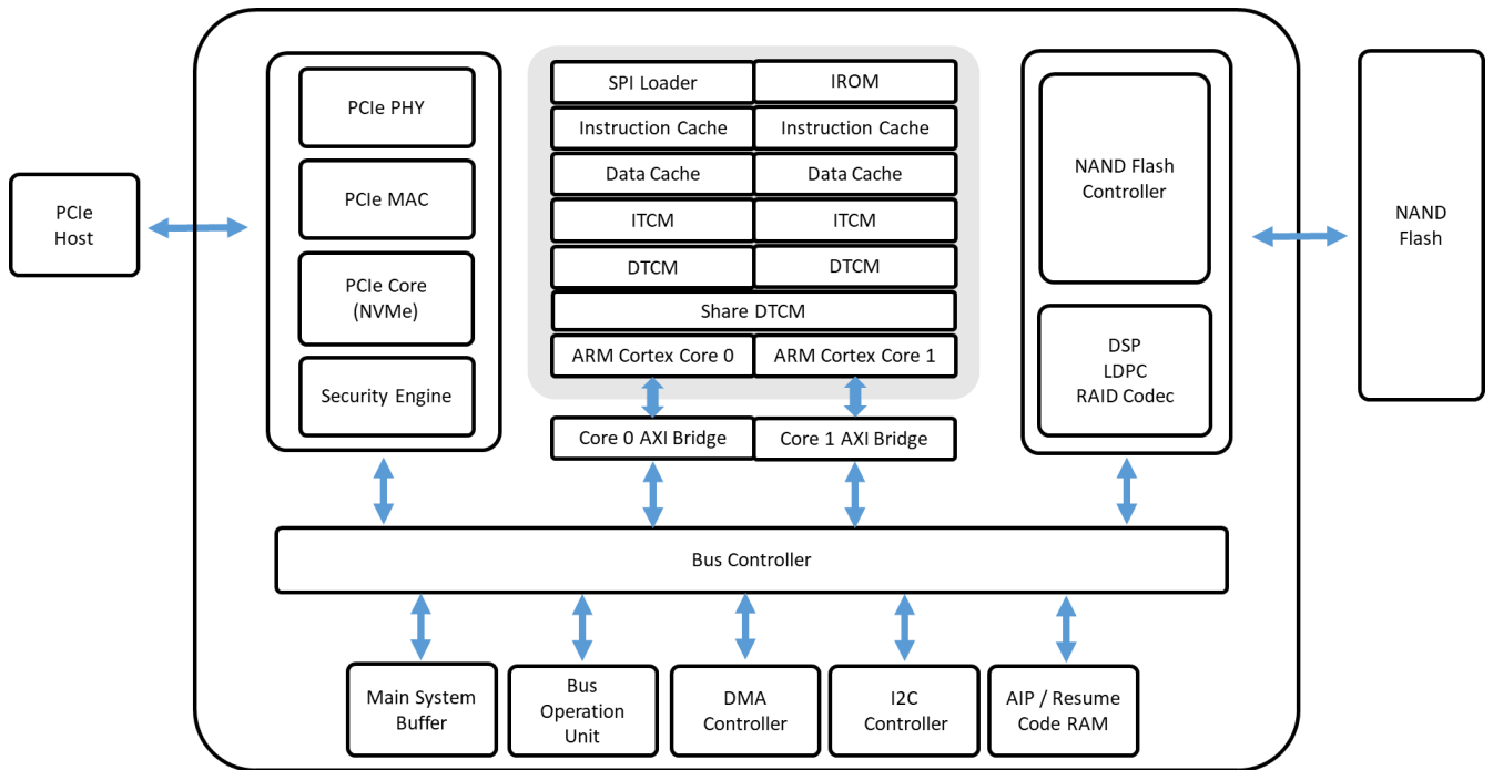
Figure 3: Innodisk M.2 (P80) 3TE4 Block Diagram
