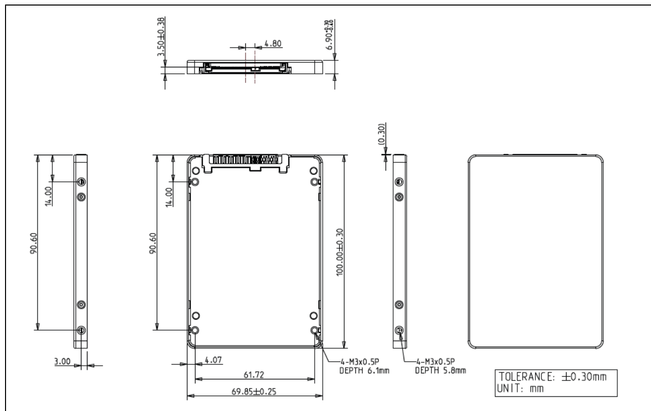
Figure 2: Innodisk U.2 SSD 4TG2-P
