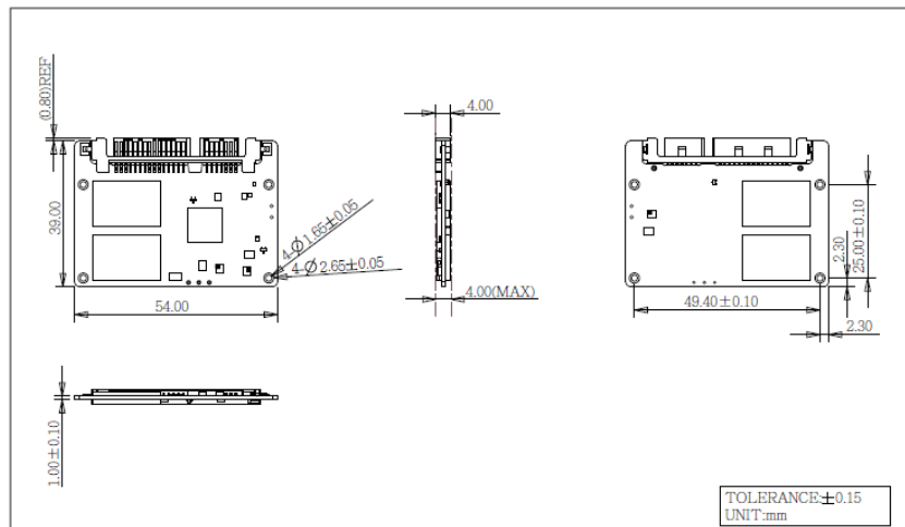
Figure 2 : SATA Slim PCBA diagram
