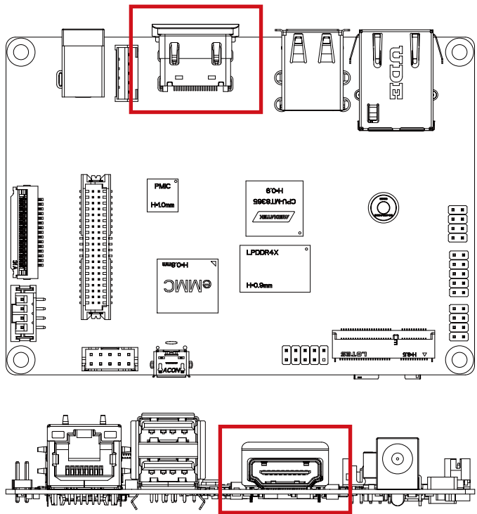
HDMI Connector
