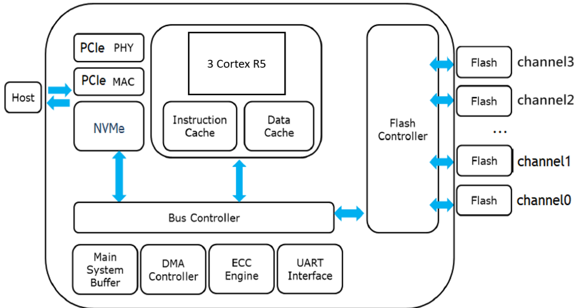
Figure 3: Innodisk M.2 (P42) 4TE2 Block Diagram
