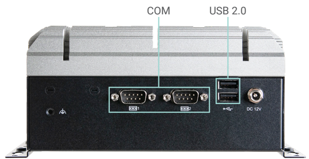
Rear View ES220F-CS (3 Storage)
