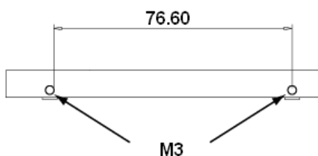
Figure 6: 2.5" SATA SSD 3TG8-P Mechanical Screw Hole
