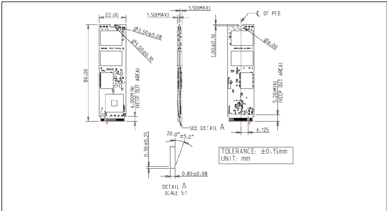
Figure 5: Innodisk M.2 (P80) 4TG2-P
