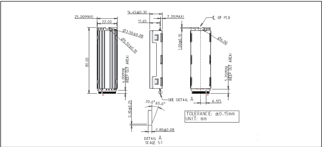
Figure 4: Innodisk M.2 (P80) 4TG2-P with heatsink diagram
