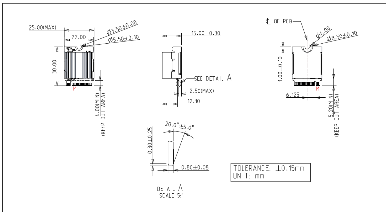
Figure 4: Innodisk M.2 (P30) 4IE3 mechanical drawing with heatsink diagram
