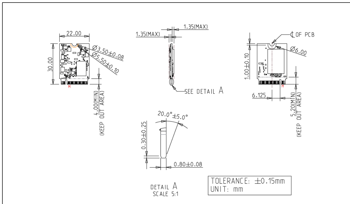
Figure 3: Innodisk M.2 (P30) 4IE3 mechanical drawing
