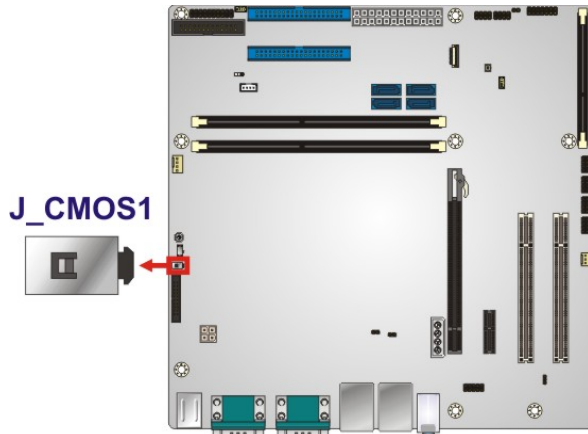
Figure 4-9: Clear CMOS Button Location
