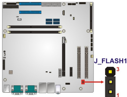
Figure 4-11: Flash Descriptor Security Override Jumper Location
