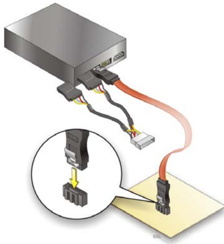
Figure 4-13: SATA Power Drive Connection
