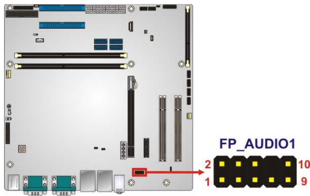
Figure 3-2: Audio Connector Location
