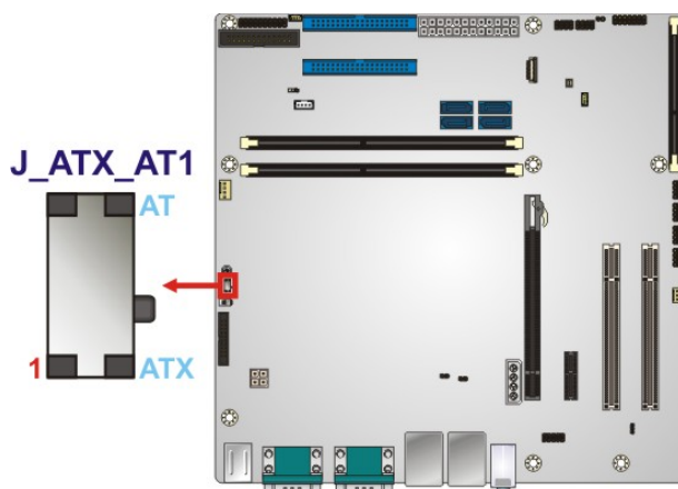
Figure 4-8: AT/ATX Power Mode Switch Location
