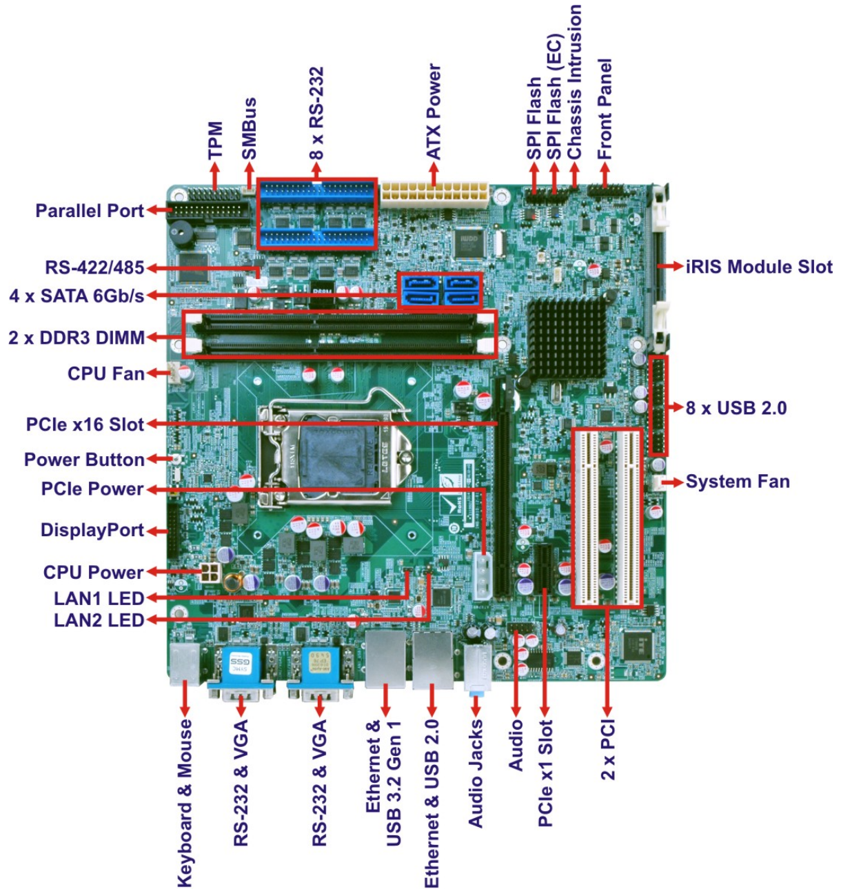
Figure 1-2: Connectors
