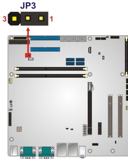
Figure 4-10: COM 10 Function Select Jumper Location
