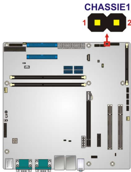
Figure 3-5: Chassis Intrusion Connector Location
