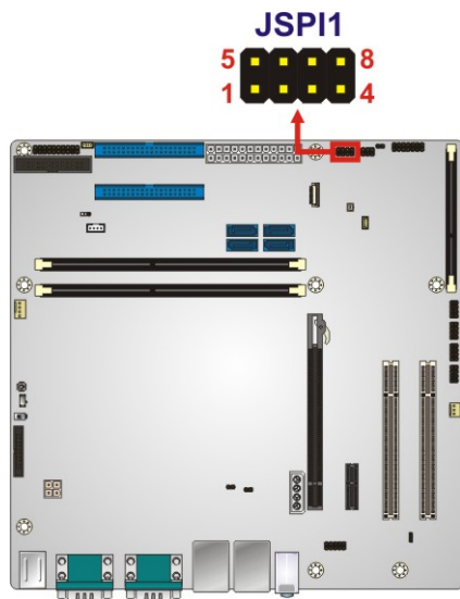
Figure 3-22: SPI Flash Connector Location
