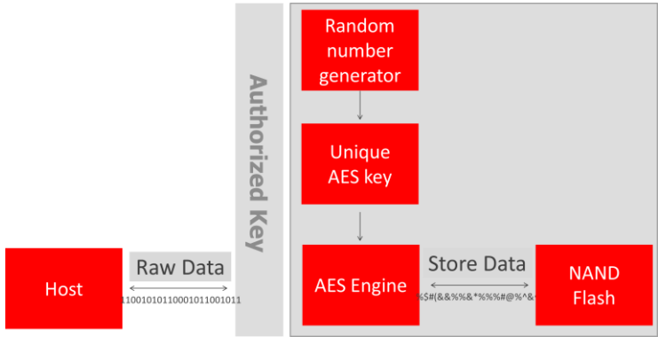
Figure 4: Innodisk 2.5" SATA SSD 3TG6-P AES flow chart
