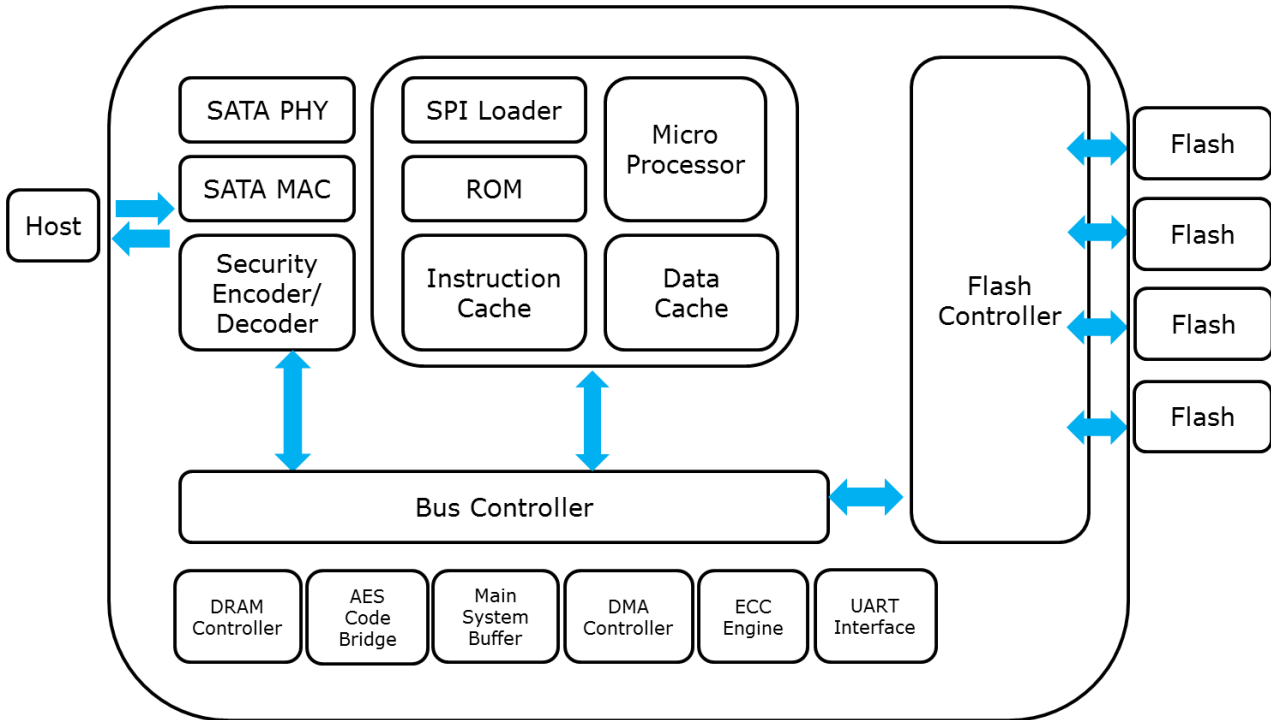
Figure 2: Innodisk 2.5" SATA SSD 3TG6-P with AES Block Diagram
