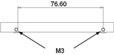
Figure 6: 2.5" SATA SSD 3TG6-P Mechanical Screw Hole
