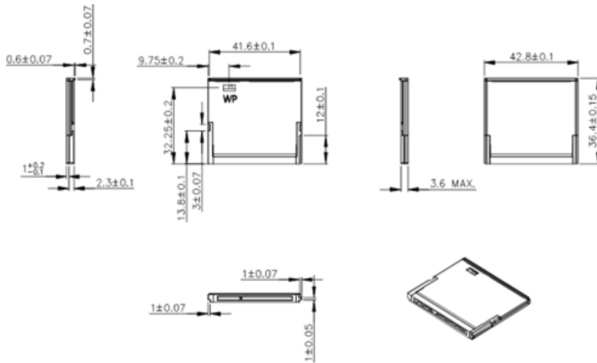
Figure 2: Innodisk CFast 3TE7 diagram
