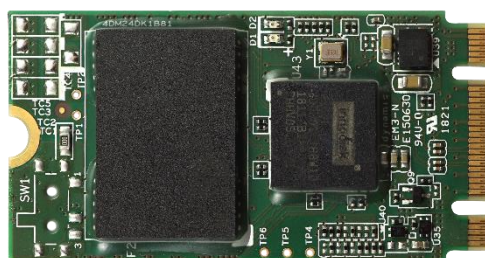
Figure 1: Innodisk M.2 (S42) 3TE7 (type 2242)
