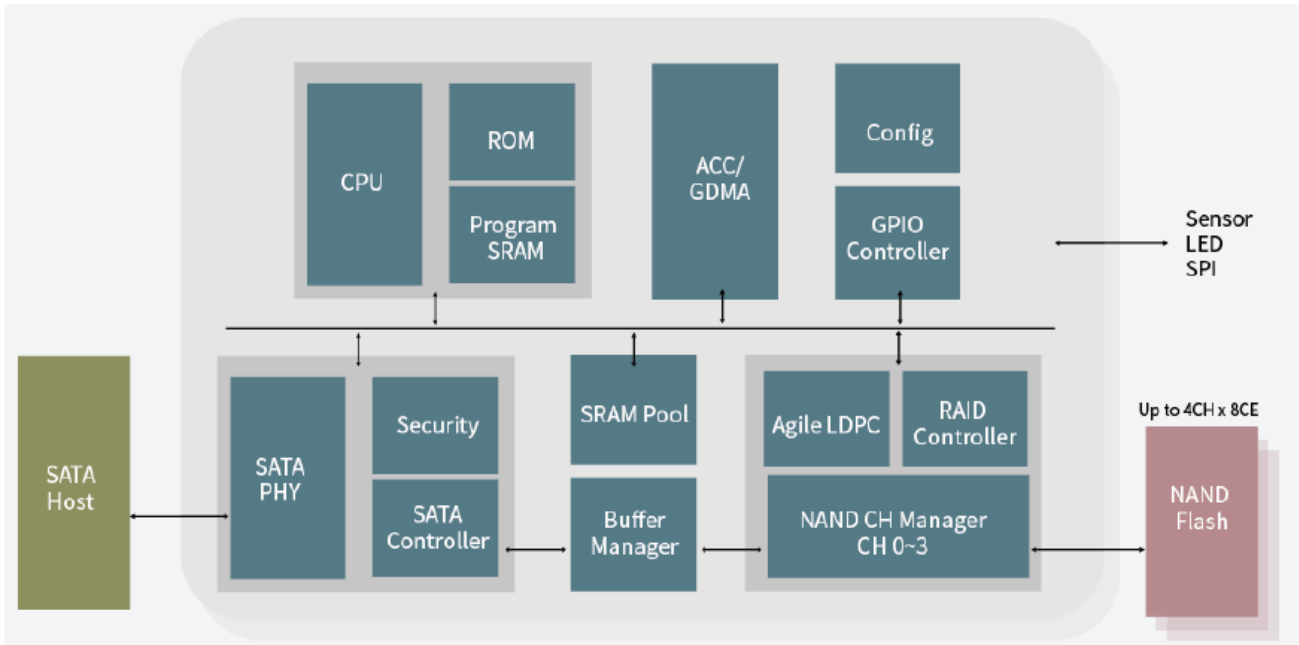
Figure 3: Innodisk M.2 (S42) 3TE7 Block Diagram
