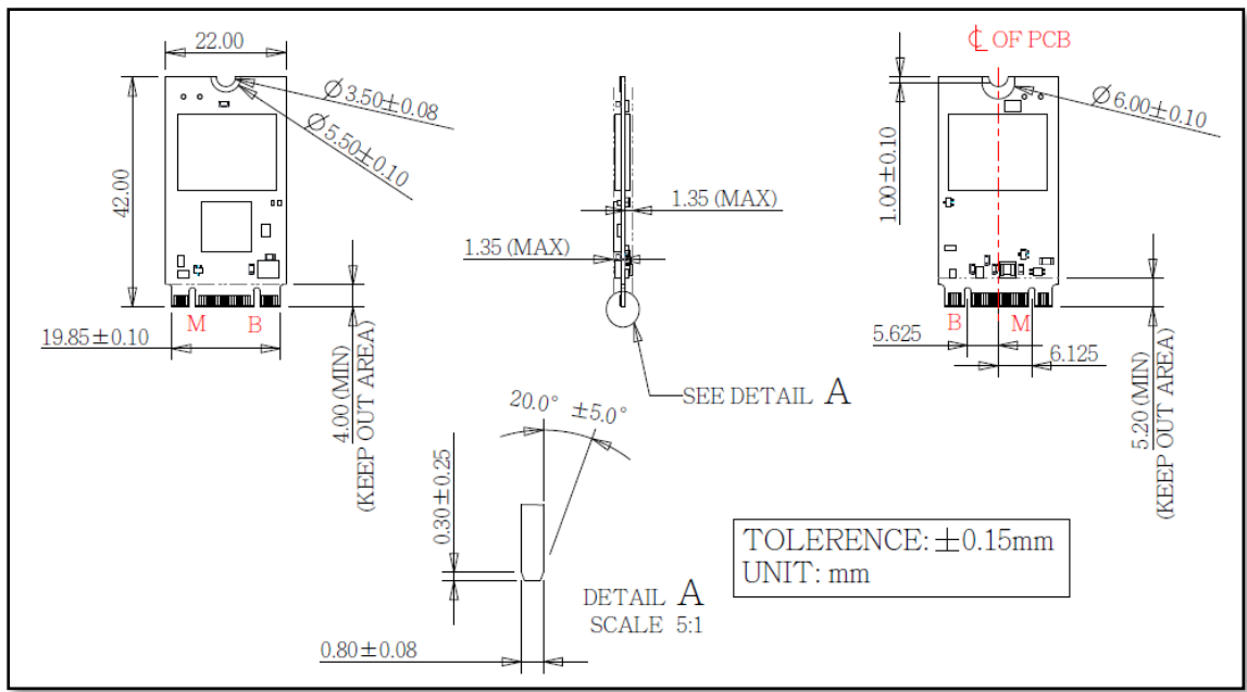
Figure 2: Innodisk M.2 (S42) 3TE7 diagram (BGA)
