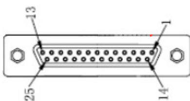
Figure 2.7 DIO Connector
