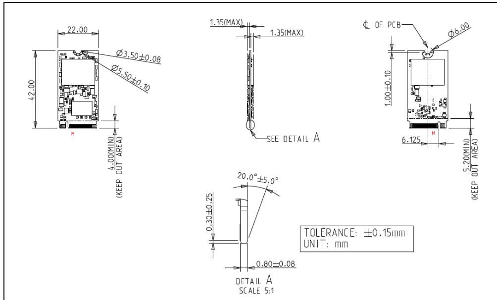
Figure 2: Innodisk M.2 (P42) 4TE2 mechanical drawing
