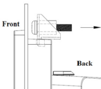
Fasten the Hook Bracket
