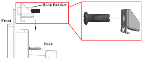
Hook brackets for panel mounting
