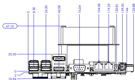
Figure 1.4 MIO-5393 Mechanical Drawing (with Cooler)
