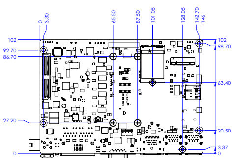
Figure 1.3 MIO-5393 Mechanical Drawing (Coastline)
