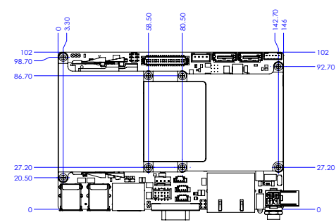
Figure 1.5 MIO-5393 Mechanical Drawing (with Heatsink)
