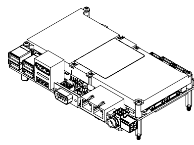
Figure 1.6 MIO-5393 Mechanical Drawing (with Heat Spreader)
