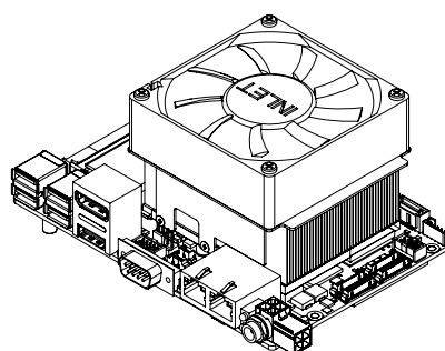
Figure 1.4 MIO-5393 Mechanical Drawing (with Cooler)
