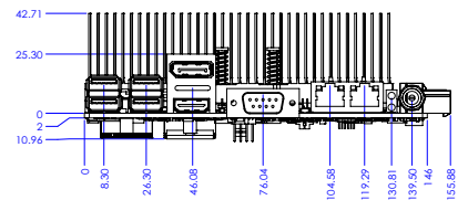
Figure 1.5 MIO-5393 Mechanical Drawing (with Heatsink)
