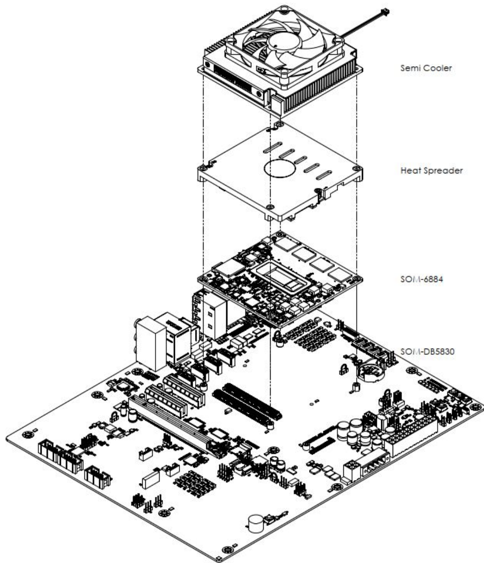
Figure 2.12 A2 Version Assembly Diagram
