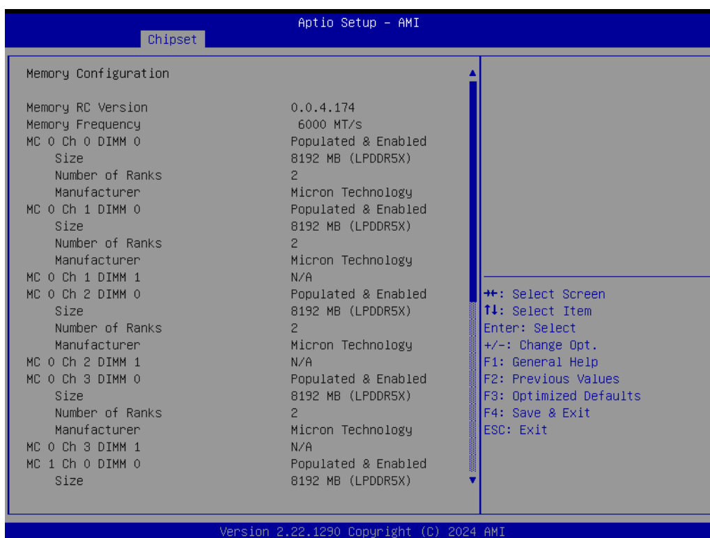
Figure 3.27 A2 Version Memory Configuration
