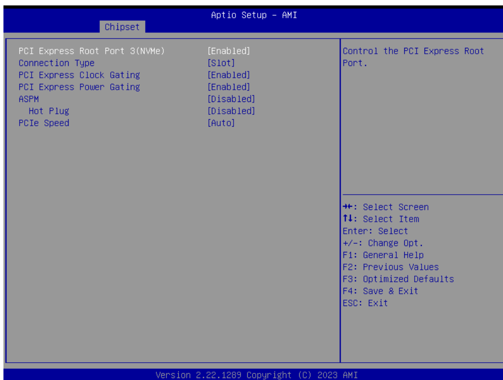
Figure 3.35 PCI Express Root Port 3 (NVME)
