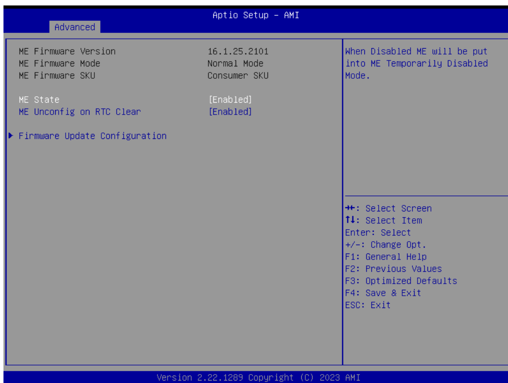
Figure 3.10 ME FW Configuration
