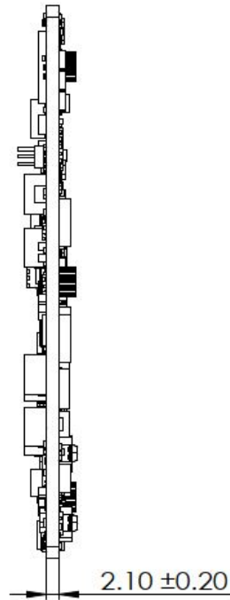
Figure 2.10 A2 Version Board Mechanical Diagram – Side1
