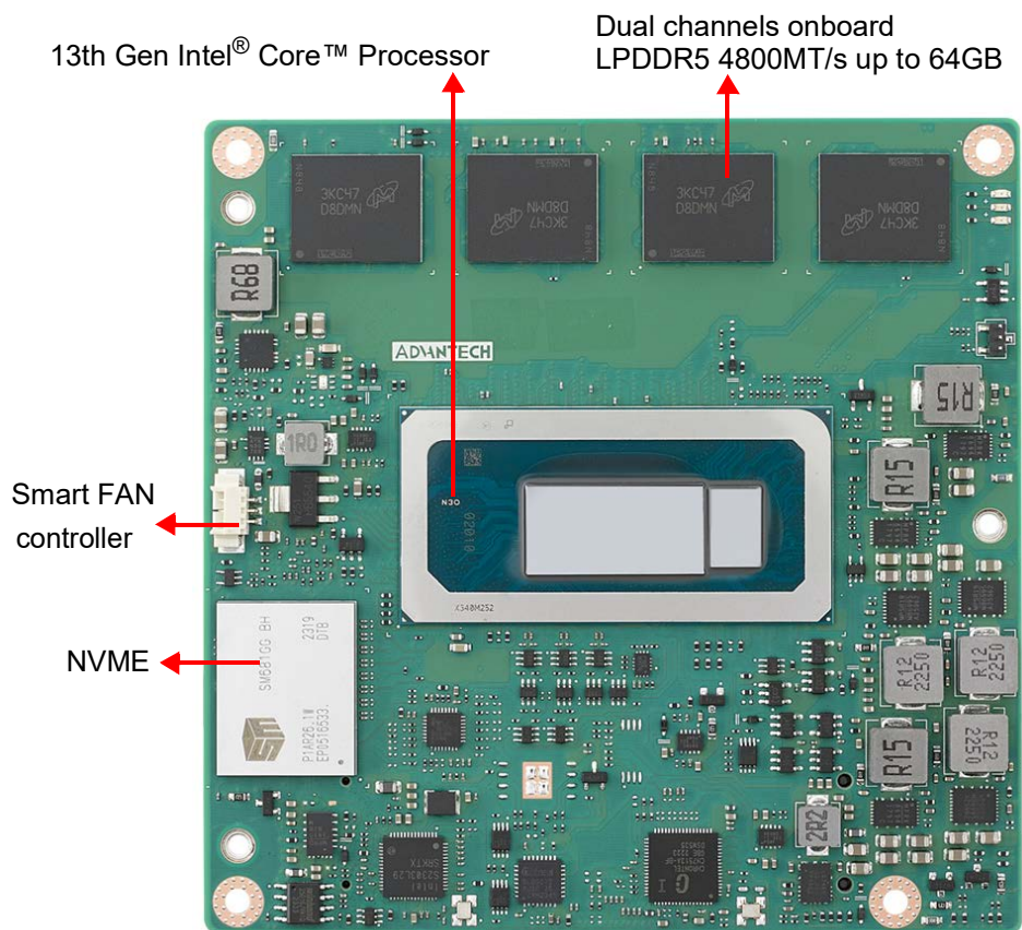
Figure 2.3 A2 Version Board Chips ID – Front
