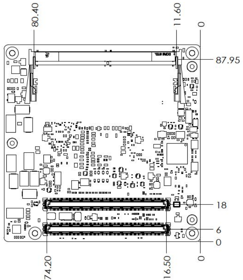
Figure 2.6 A1 Version Board Mechanical Diagram – Rear
