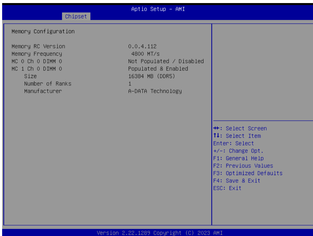
Figure 3.26 A1 Version Memory Configuration
