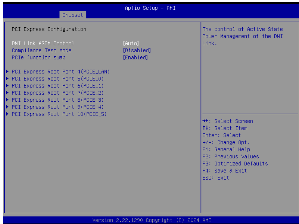
Figure 3.32 A2 Version PCI Express Configuration
