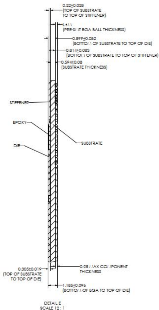
Figure 2.13 CPU Height and Tolerance
