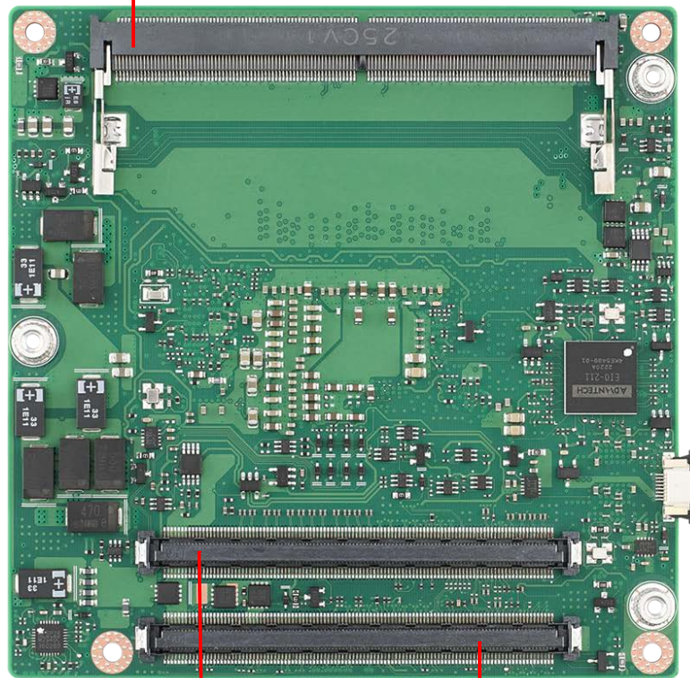
Figure 2.2 A1 Version Board Chips ID – Rear
