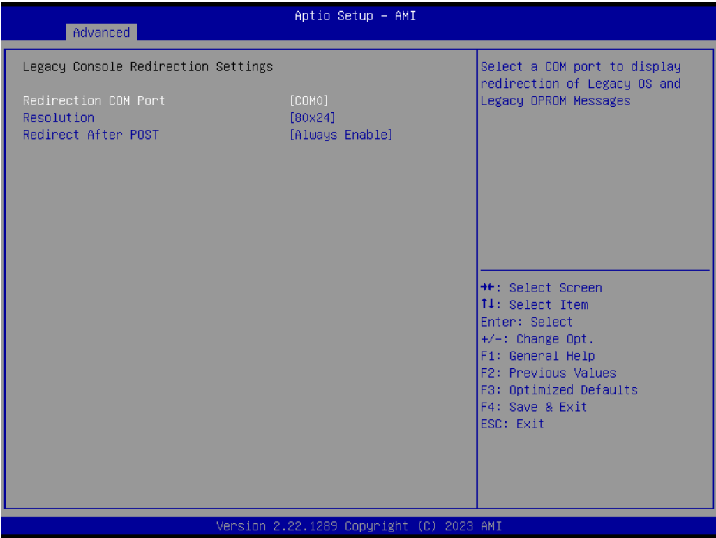
Figure 3.17 Legacy Console Redirection Settings
