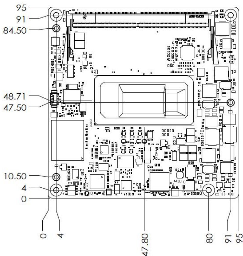
Figure 2.5 A1 Version Board Mechanical Diagram - Front
