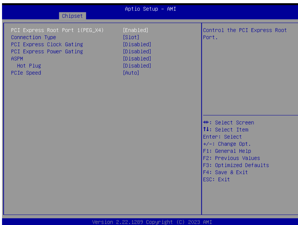
Figure 3.33 PCI Express Root Port 1 (PEG_4)
