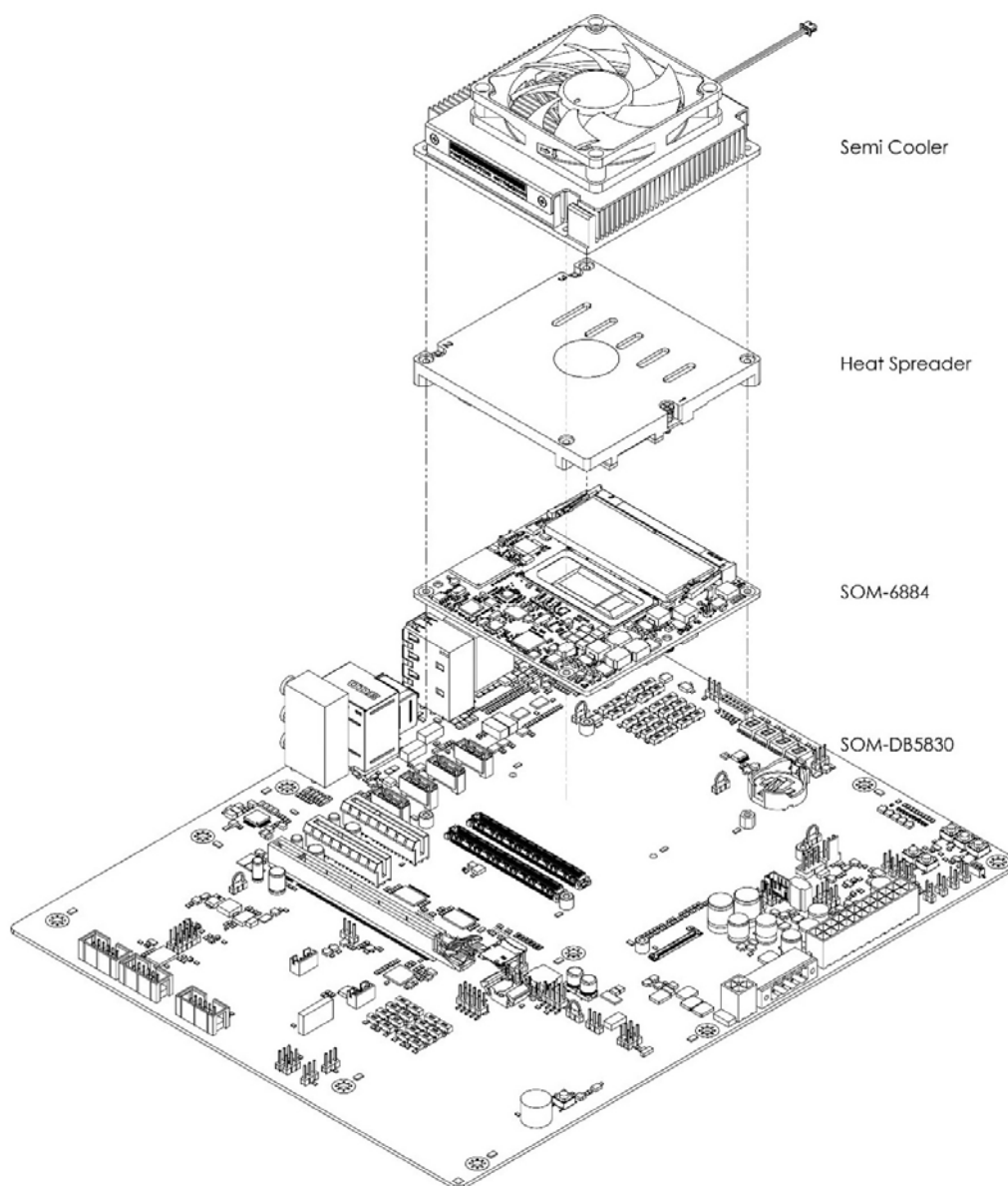
Figure 2.11 A1 Version Assembly Diagram
