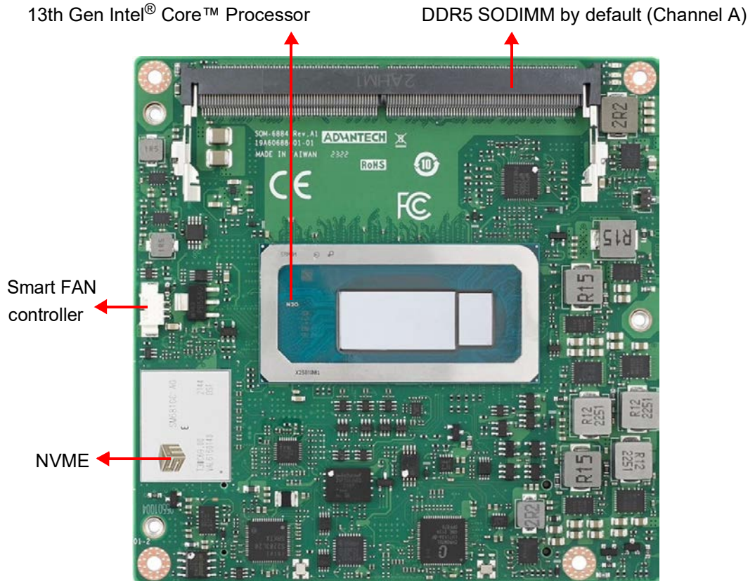
Figure 2.1 A1 Version Board Chips ID – Front
