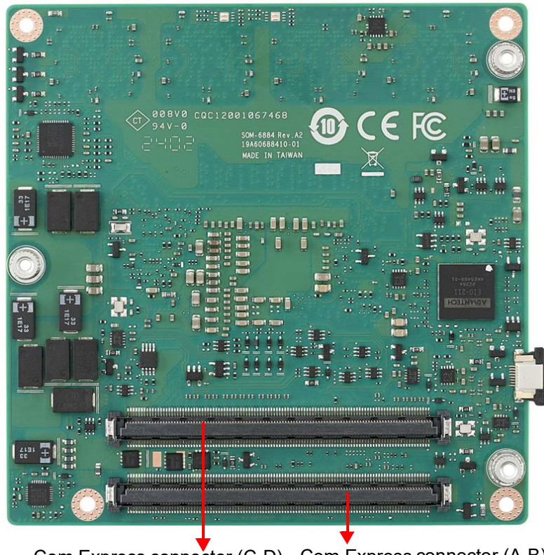
Figure 2.4 A2 Version Board Chips ID – Rear
