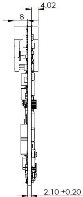
Figure 2.7 A1 Version Board Mechanical Diagram – Side1
