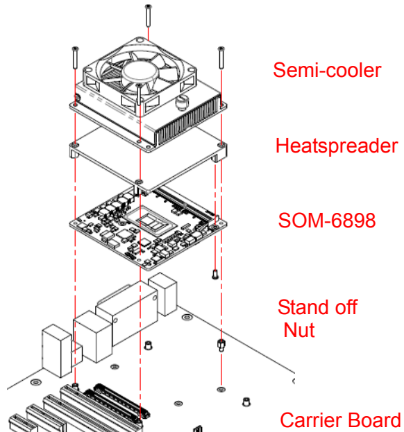
Figure 2.5 Assembly Drawing
