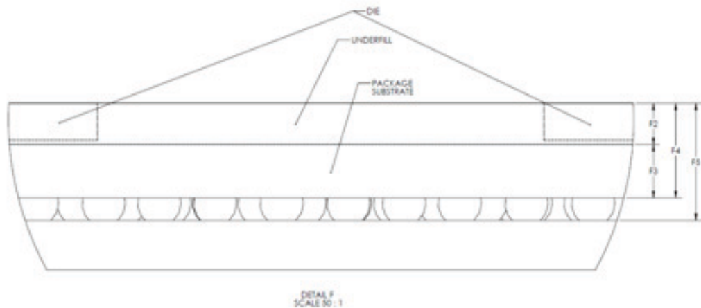
Figure 2.6 Main Chip Height and Tolerance (GT2)
