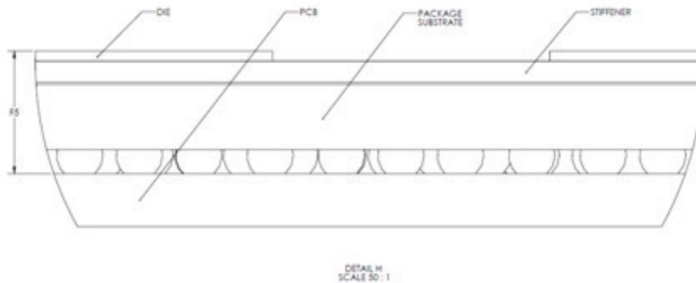
Figure 2.7 Main Chip Height and Tolerance (GT3)
