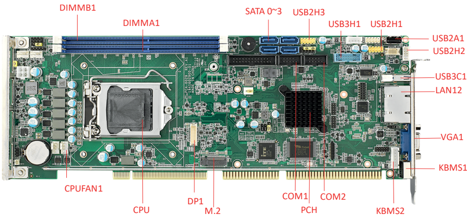
Figure 1: Board Layout: Jumper and Connector Locations
