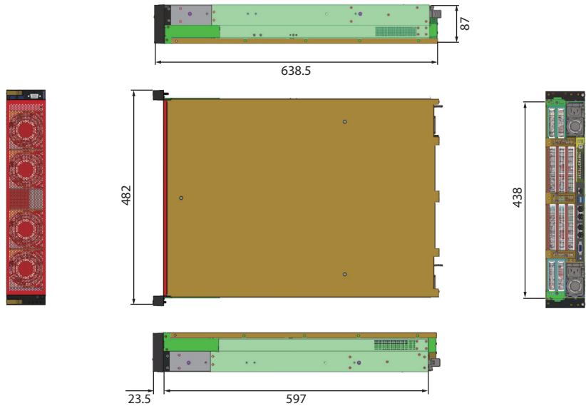
Front View (w/optional bezel)
