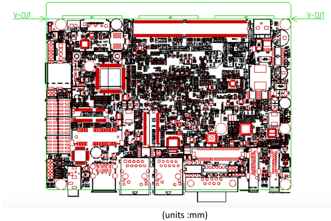
Figure 2.1: Board Dimension of SBC-7127
