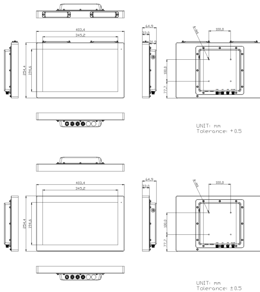
Figure 1 Dimensions of PHANTAM-816BP/BR(H)
