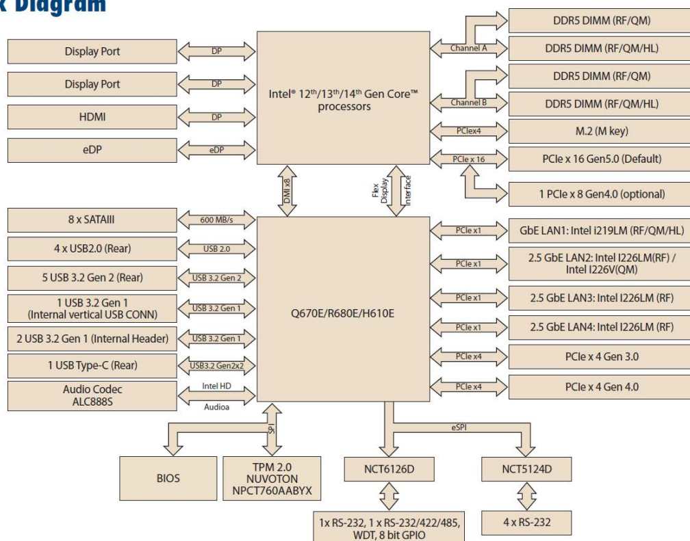
Figure 1.3 AIMB-588 B1 Block Diagram
