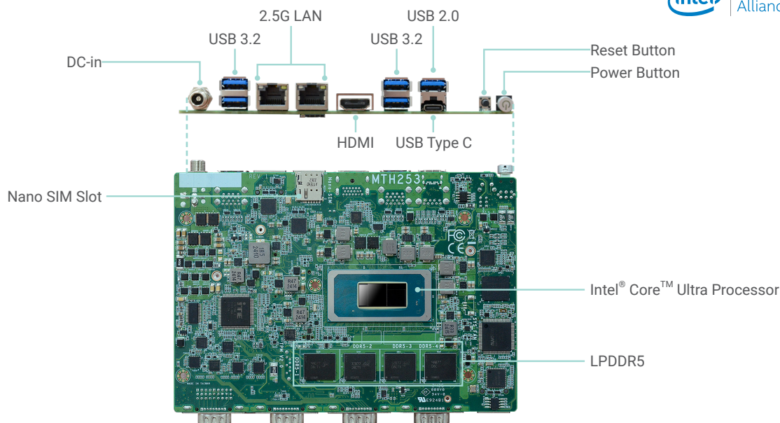
Bottom View
