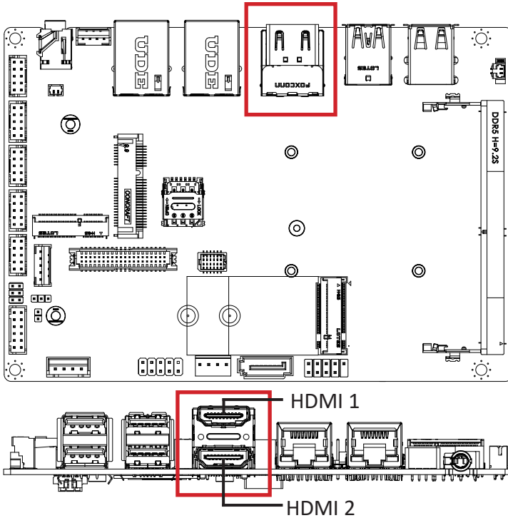
HDMI Connector
