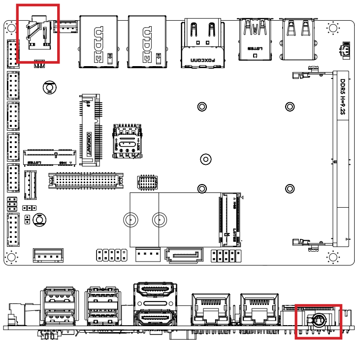
Audio Connector
