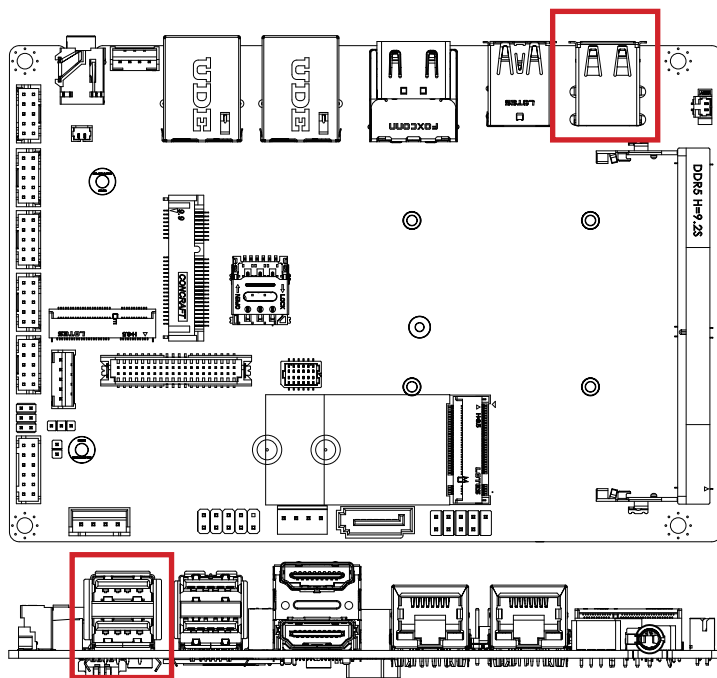
USB Connector
