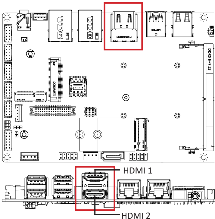
HDMI Connector
