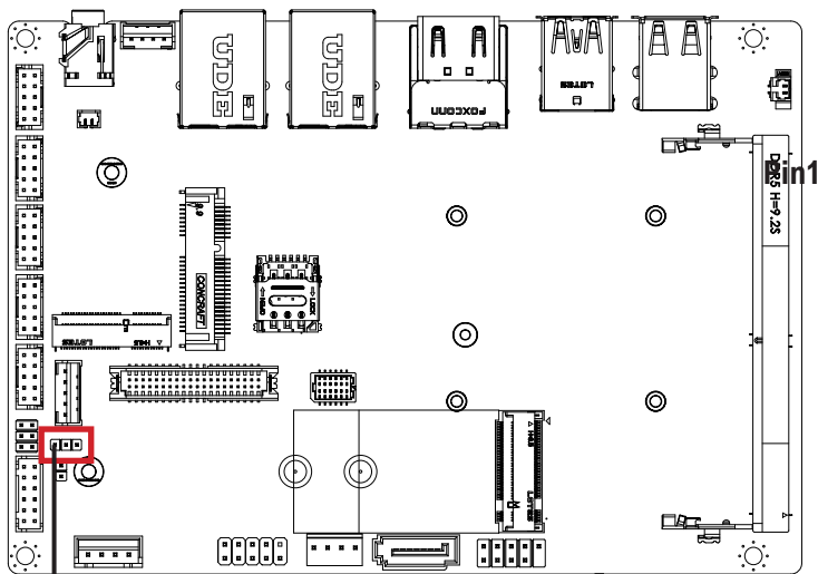
Pin 1
