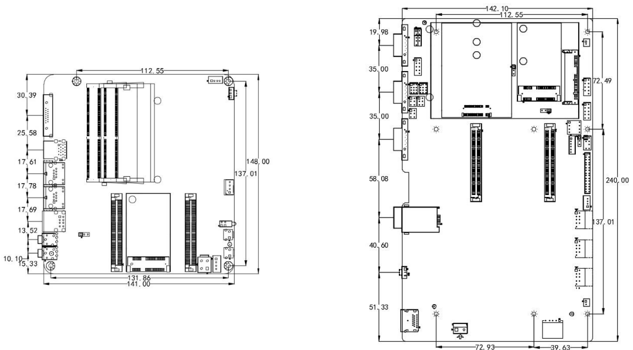
Figure 1 3.2 Main board size diagram
