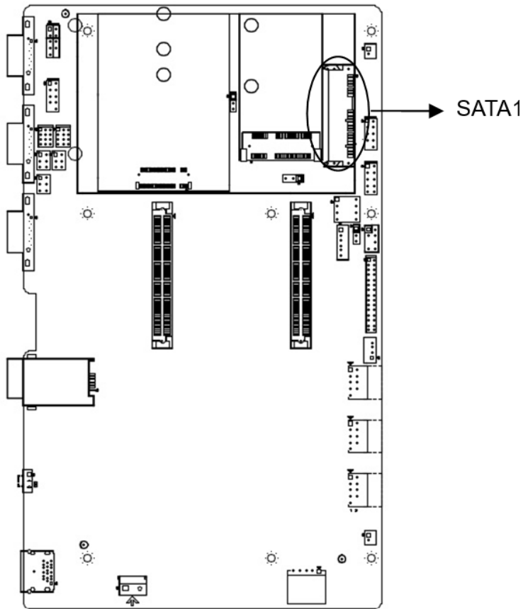
Definition of SATA1 (2.5-inch hard drive interface)
