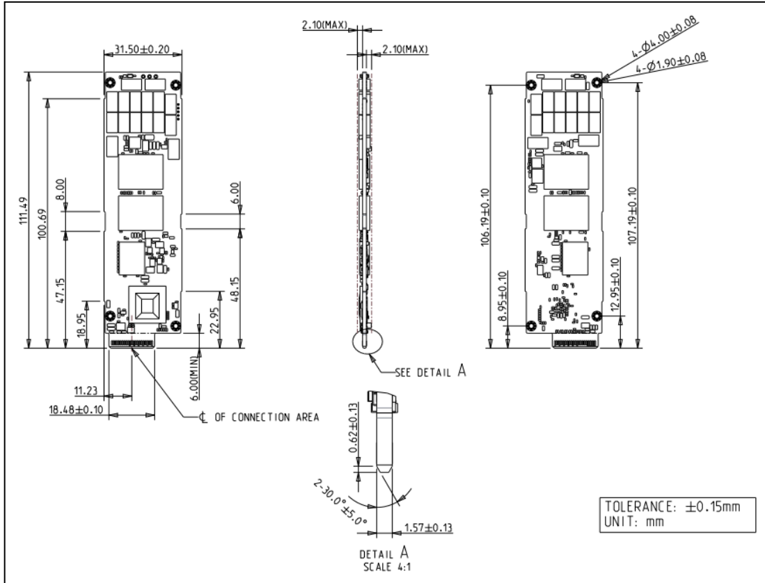
Figure 4: Innodisk E1.S 4TS2-P 5.9mm (480GB~1.92TB)
