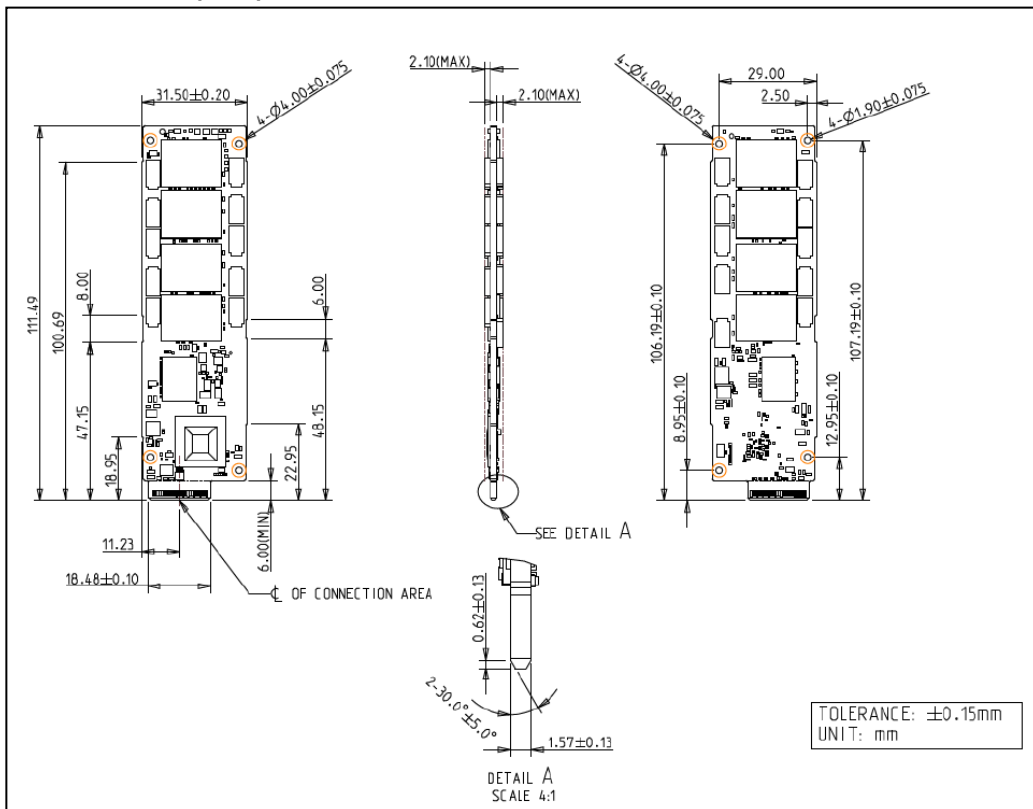
Figure 5: Innodisk E1.S 4TS2-P 5.9mm (3.84TB)
