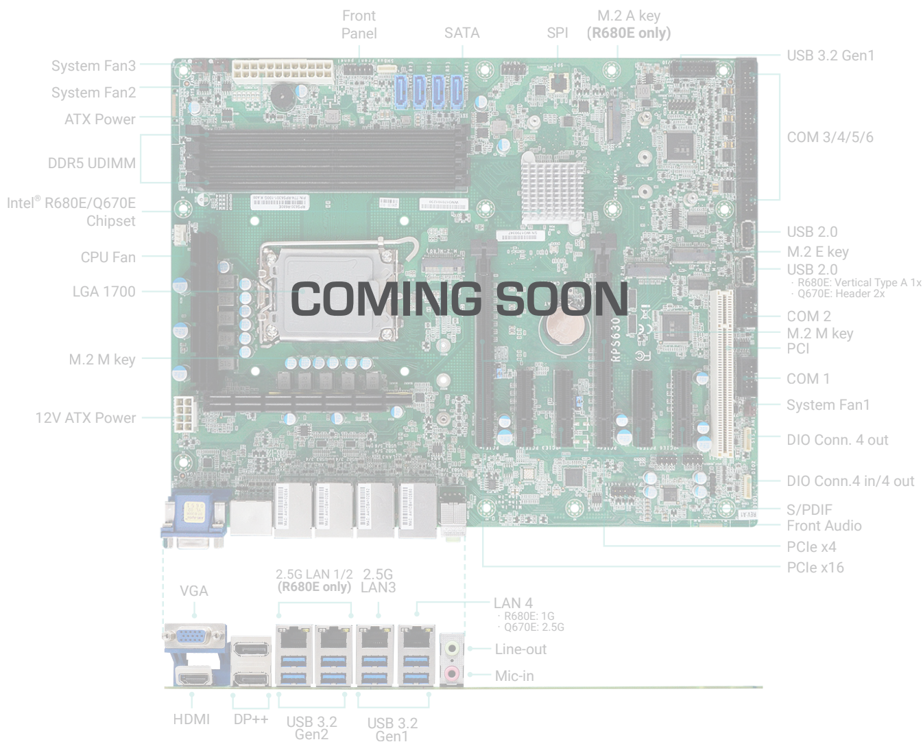
Top View (RPS630-R680E)
