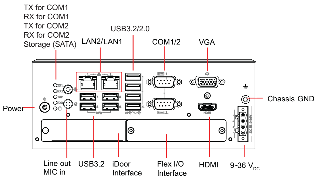
Figure 2.1 MIC-770 V3 Front View
