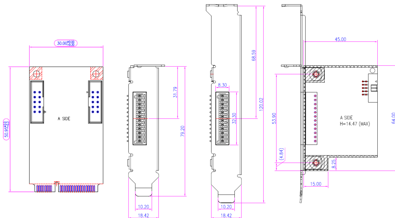
Extension board
