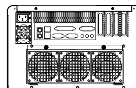
Rear View
