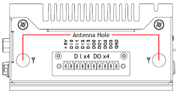
Right Side External I/O
