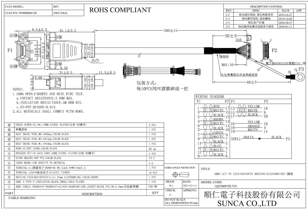
Figure 8: HDMI Cable Drawing
