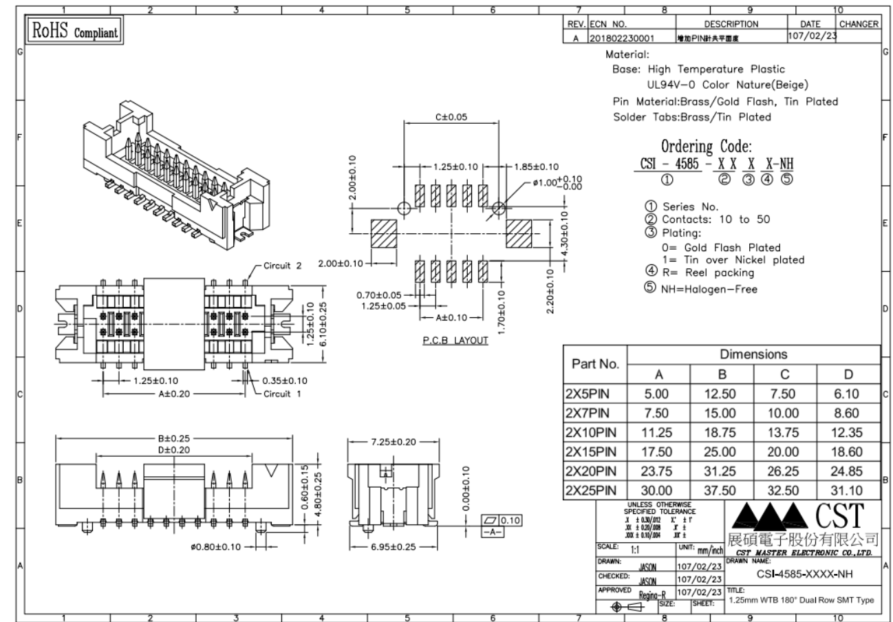
Figure 4: Wire to Board SMD 2*10P Connector Drawing (CN1/CN2/CN3)
