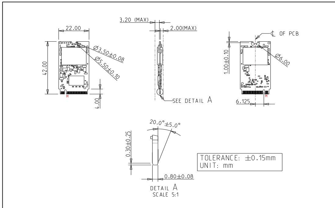
Figure 2: Innodisk M.2 (P42) 4TE2 4TB mechanical drawing
