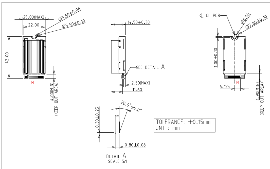
Figure 3: Innodisk M.2 (P42) 4TE2 4TB mechanical drawing with heatsink diagram
