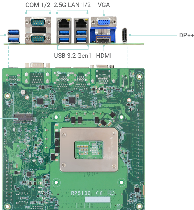
Bottom View
