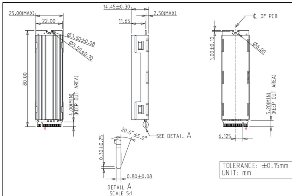
Figure 4: Innodisk M.2 (P80) 4TE2 mechanical drawing with heatsink diagram
