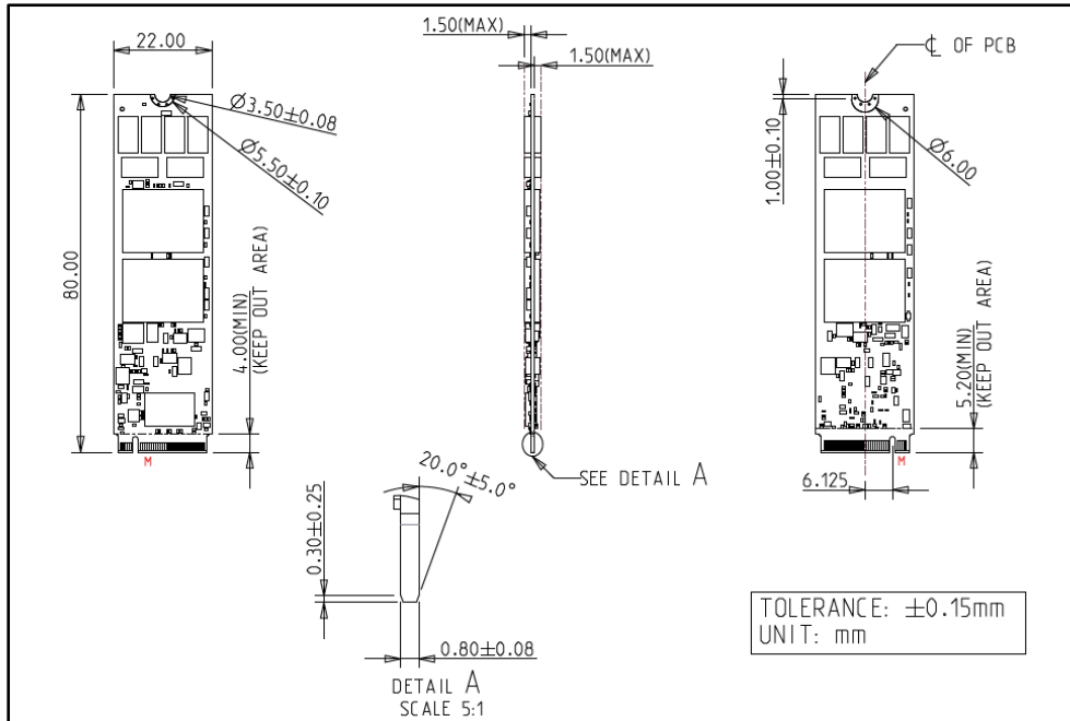
Figure 3: Innodisk M.2 (P80) 4TE2 mechanical drawing
