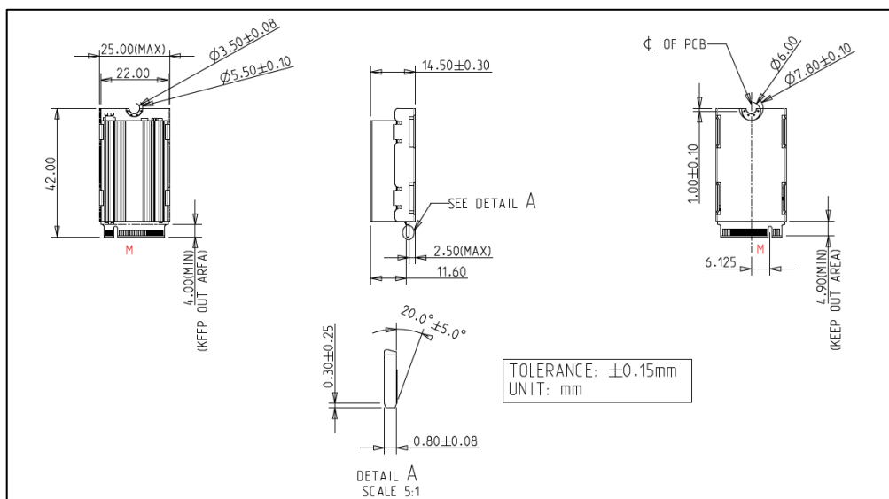
Figure 3: Innodisk M.2 (P42) 4TE2 mechanical drawing with heatsink diagram
