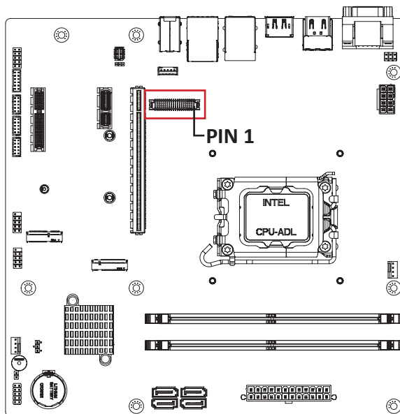
LVDS Connector
