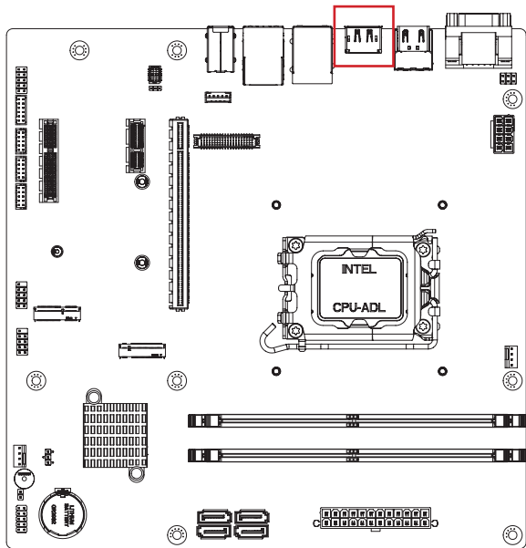
DP Connector
