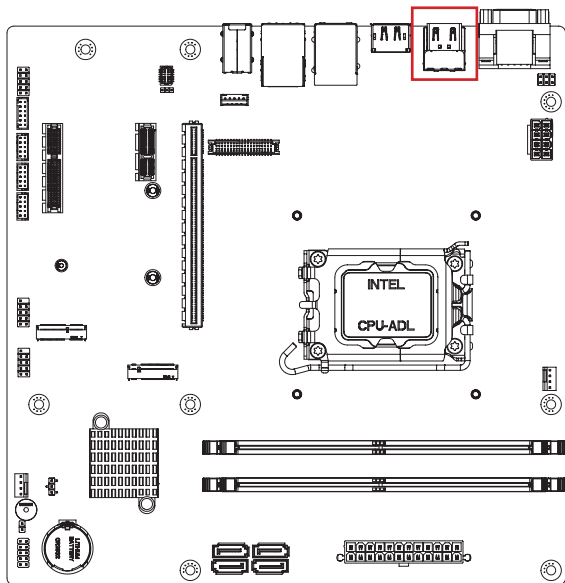
HDMI Connector
