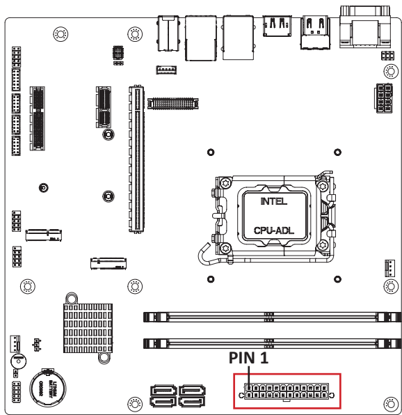
ATX power connector
