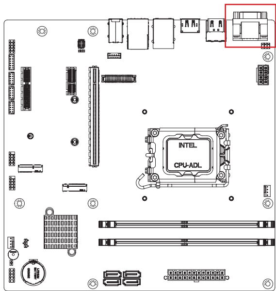
D-sub Connector
