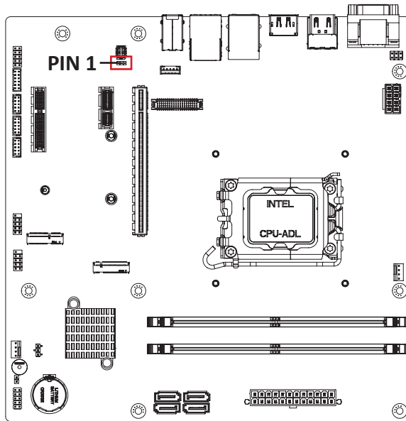
AT/ATX mode select jumper
