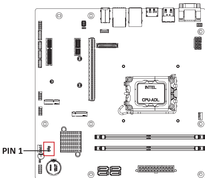
Clear CMOS connector
