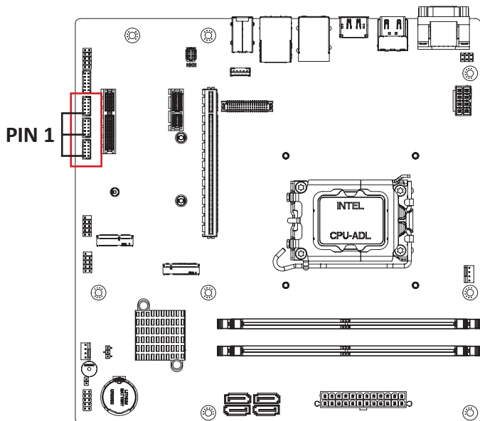
Serial port Header
