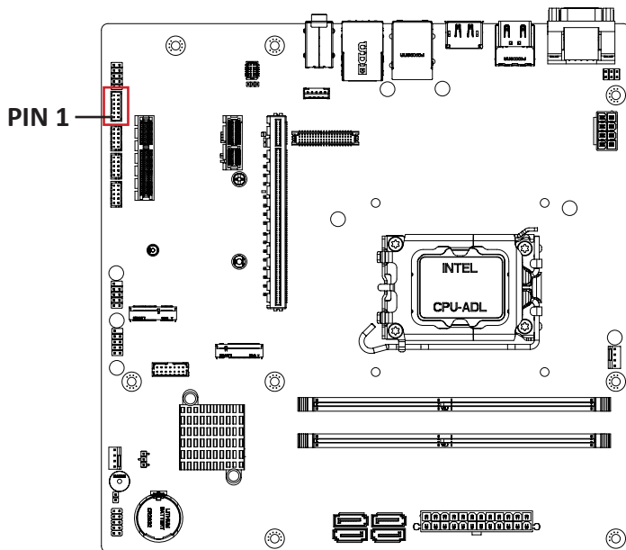
GPIO Connector
