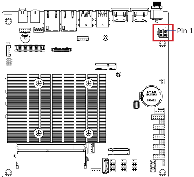
power Connector
