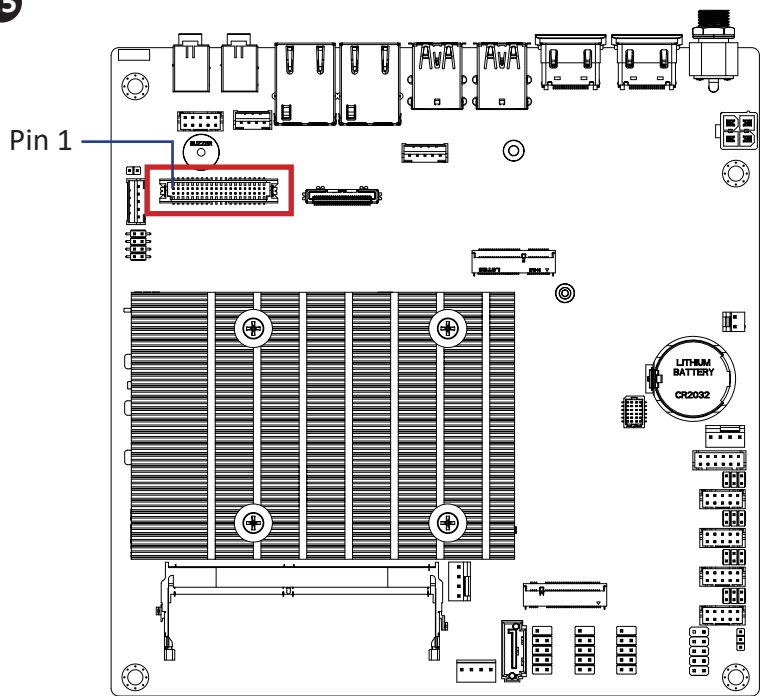
LVDS Connector
